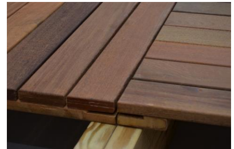
Panels on Double Stringers 24" On Center
