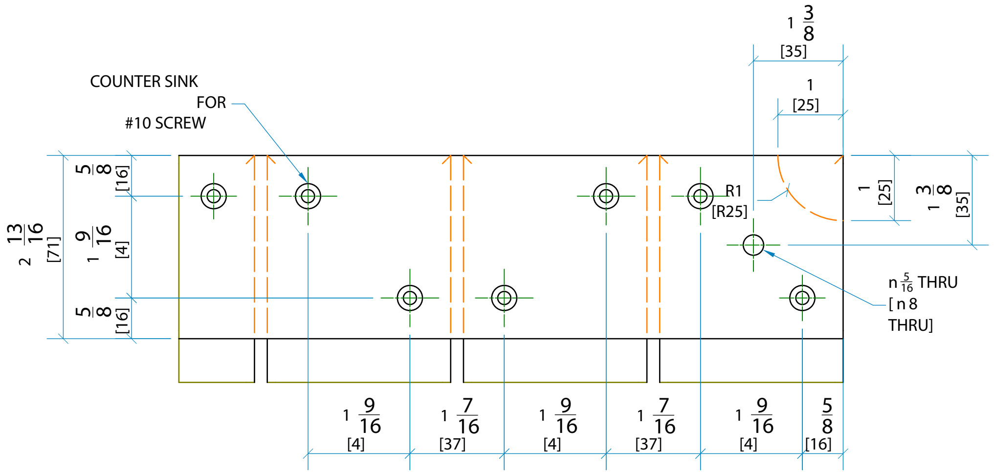
DETAIL A
