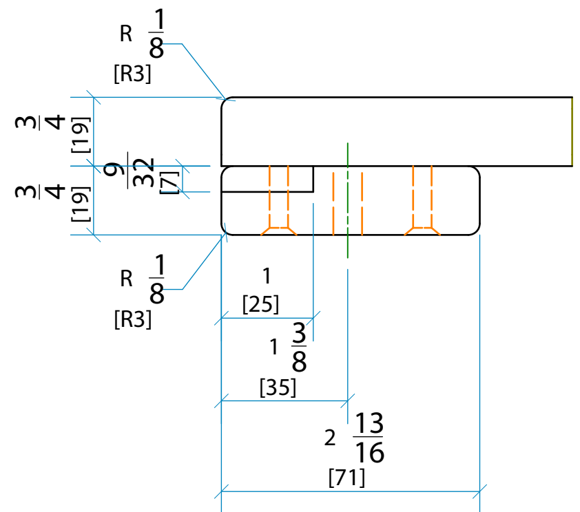
DETAIL C
