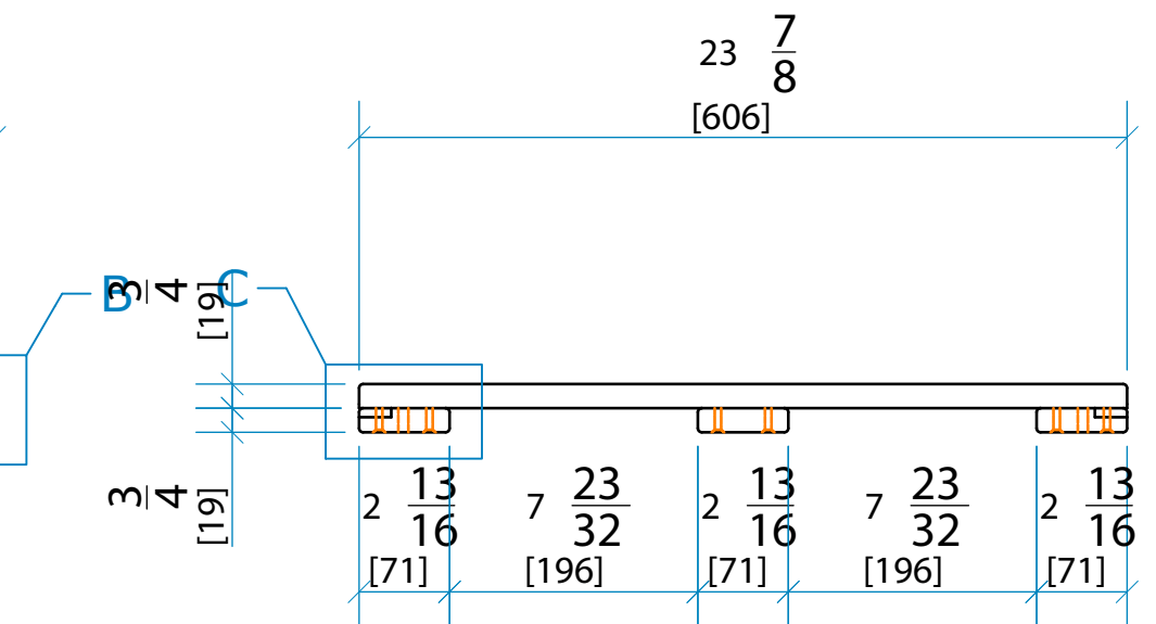
SIDE VIEW
