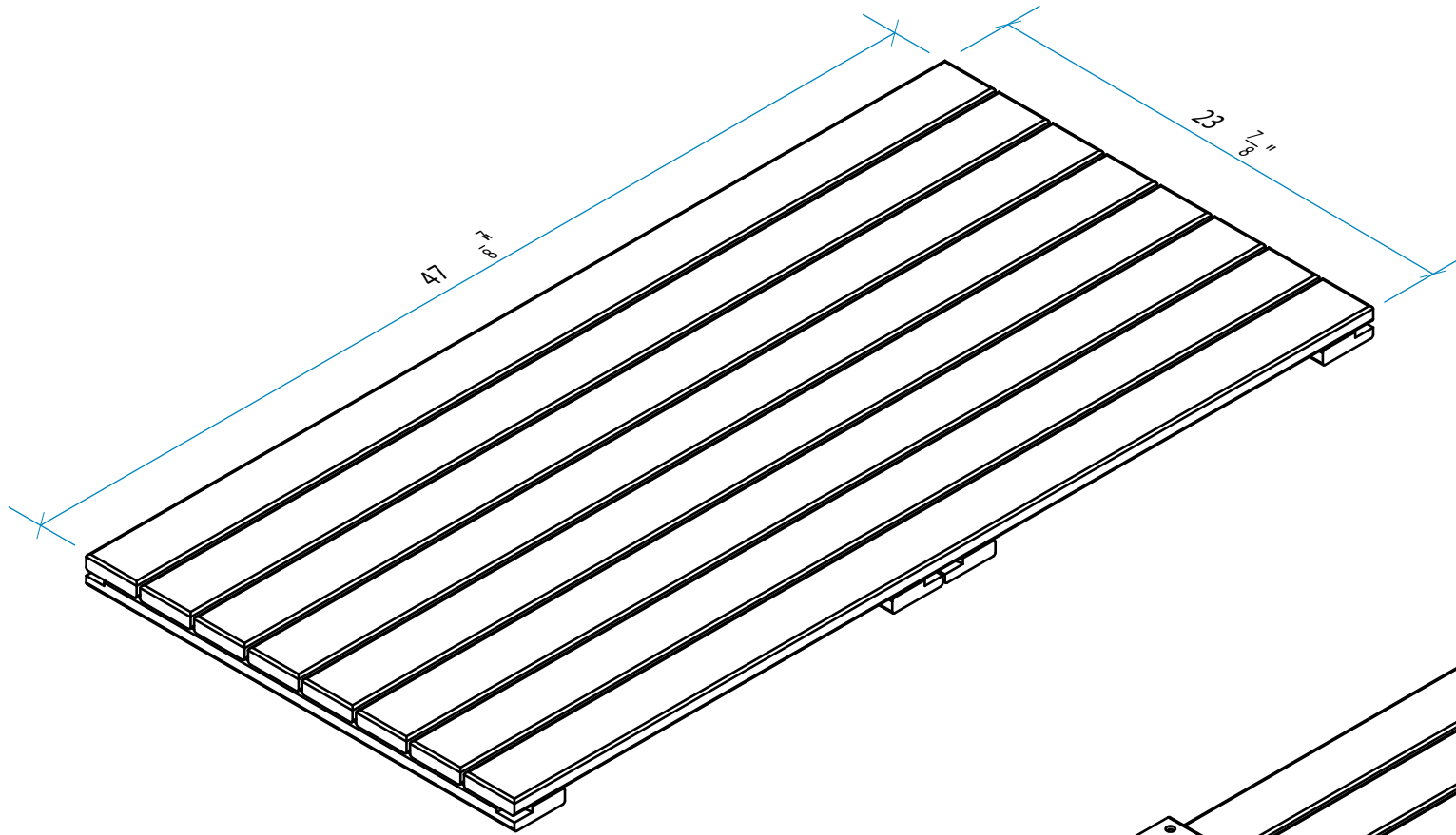
ISOMETRIC: TOP
