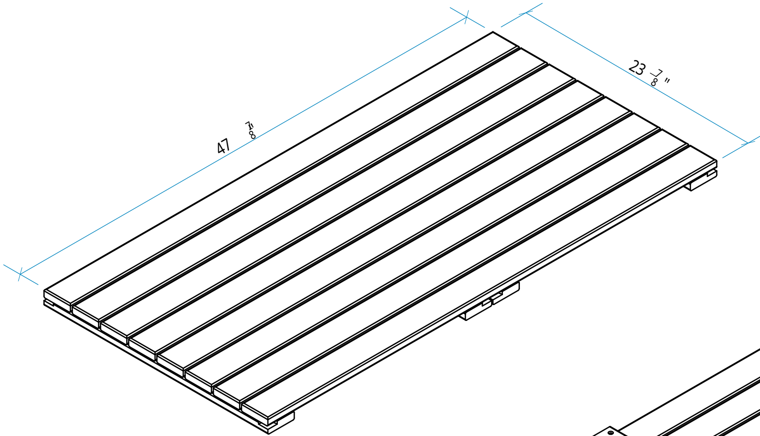
ISOMETRIC: TOP
