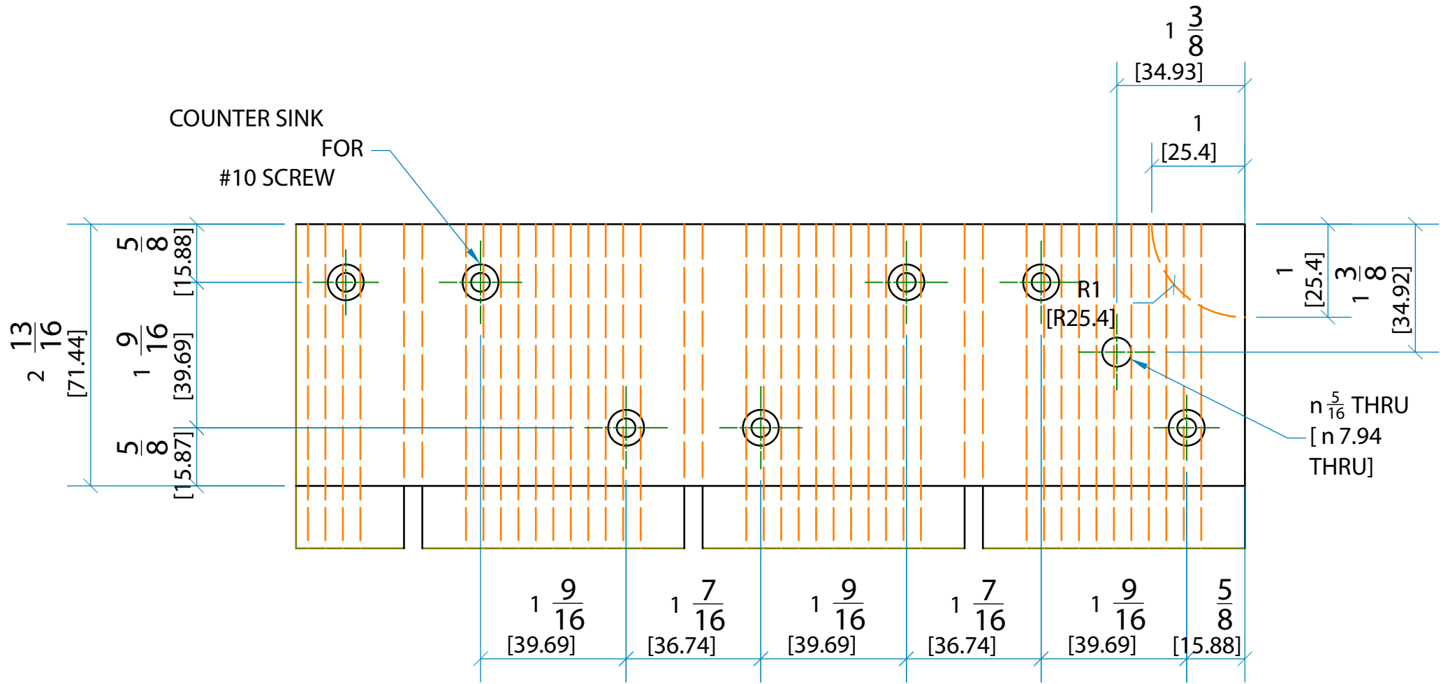
DETAIL A
