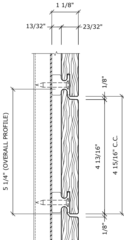
B BLACK LABEL CLAD CLIP MAXI w/ 1" X 6" 1/8 REVEAL RAINSREEN SCALE: NTS
