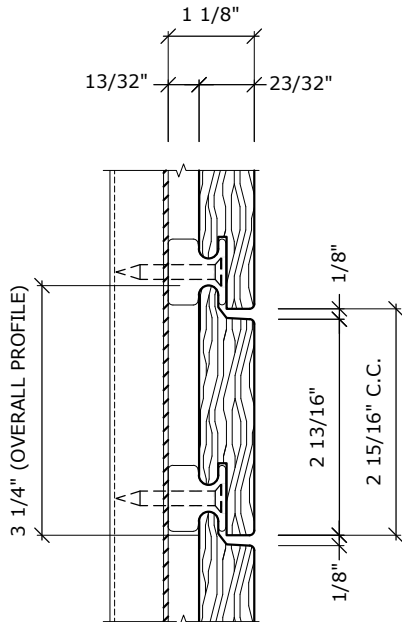
A BLACK LABEL CLAD CLIP MAXI w/ 1" X 4" 1/8 REVEAL RAINSREEN SCALE: NTS
