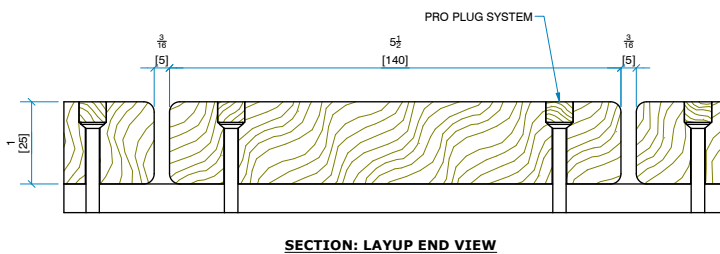
SECTION: LAYUP END VIEW
