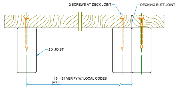
SECTION: LAYUP SIDE VIEW
