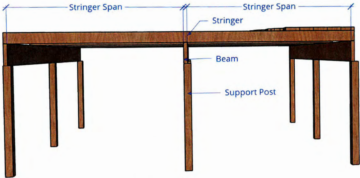
Figure 1: Stringer Span
