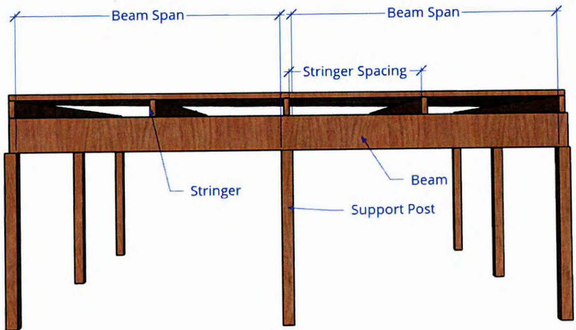
Figure 2: Beam Span
