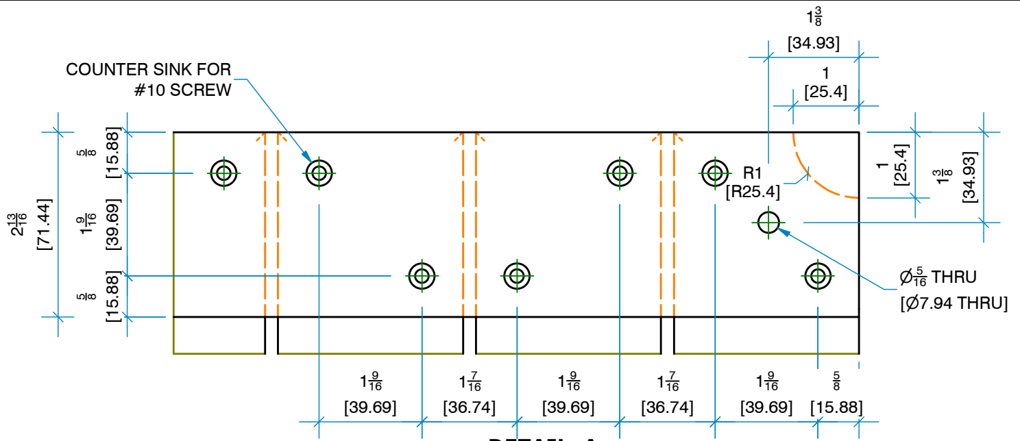
DETAIL A
