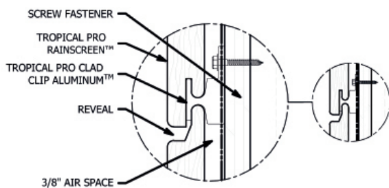
Aluminum install section detail
