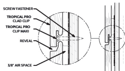
Maxi Clip install section detail
